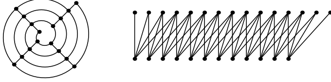
Fig. 2. R_4 and S_4
