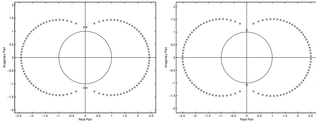
Figure 2: Distribution of the poles for k = 101 and \alpha = (k + 1)/(2k - 2) (left) and \alpha = (k + 1)/2k (right).
