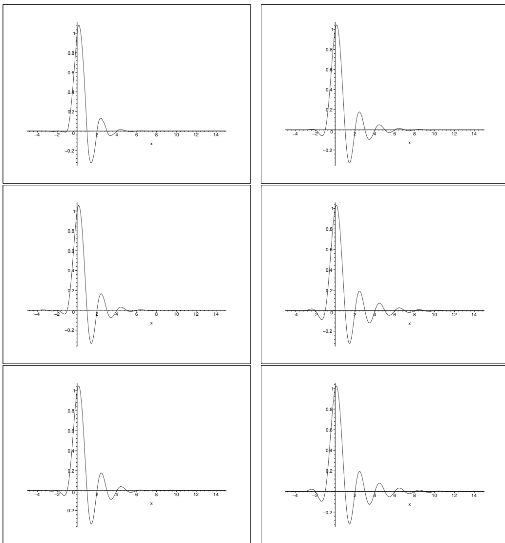
Figure 1: The refinable functions for k = 5, 9, 11 and the choices \alpha = (k + 1)/(2k - 2) (left) and \alpha = (k + 1)/2k (right).
