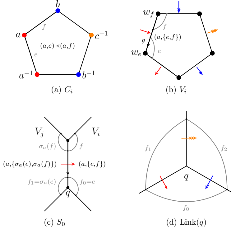
FIGURE 4. Constructing V_i and S_0 from C_i in the proof of Lemma 16. In this example, we note from (d) that f_1 = \sigma_a(f_0) , f_2 = \sigma_{c^{-1}}(f_1) and f_0 = \sigma_{b^{-1}}(f_2) .
